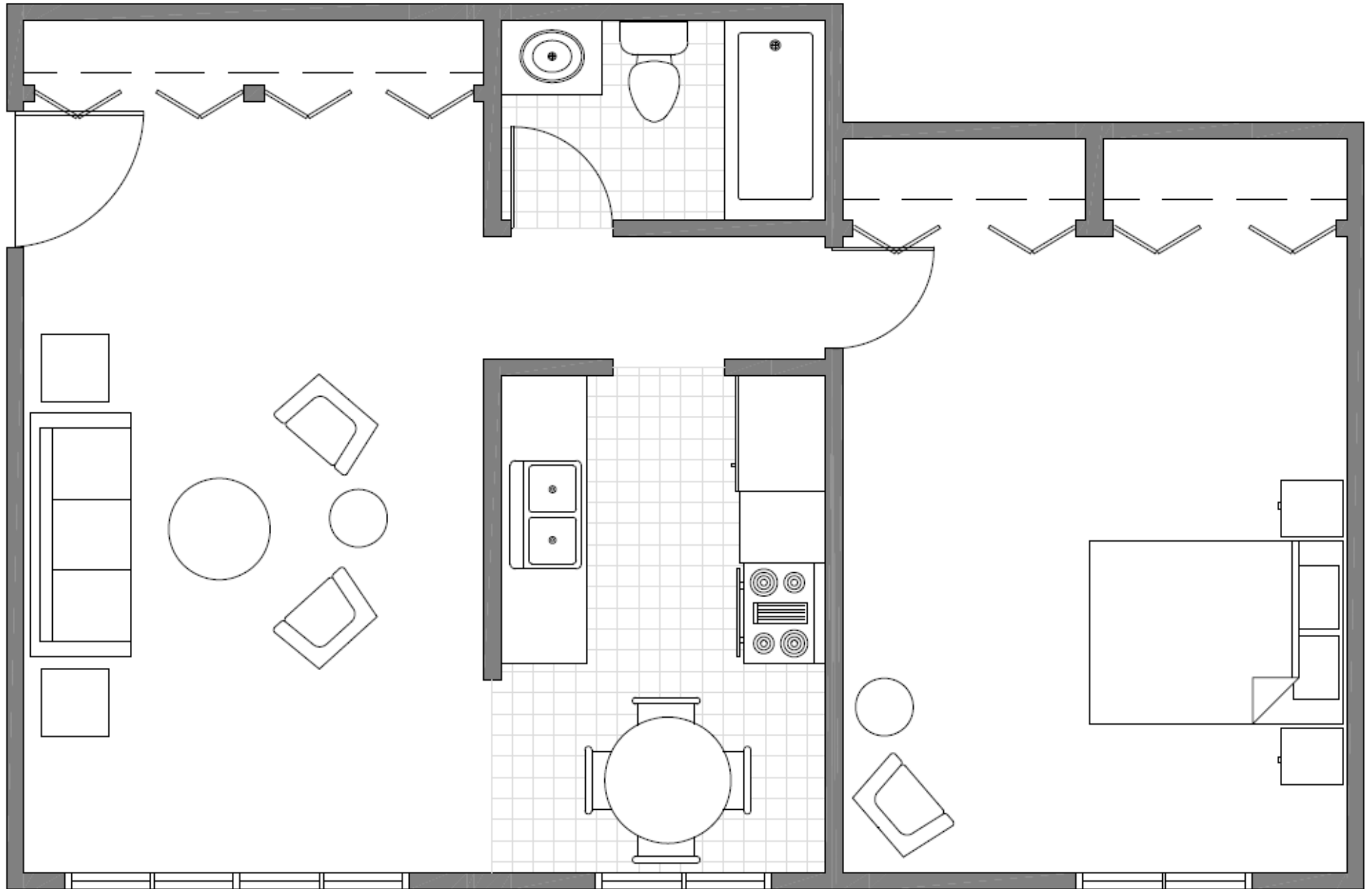
1-Bedroom Apartment
